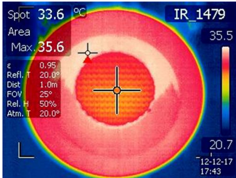
Figure 12: Thermal Image #1
