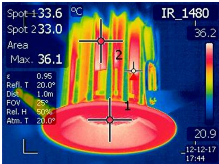
Figure 13: Thermal Image #2
