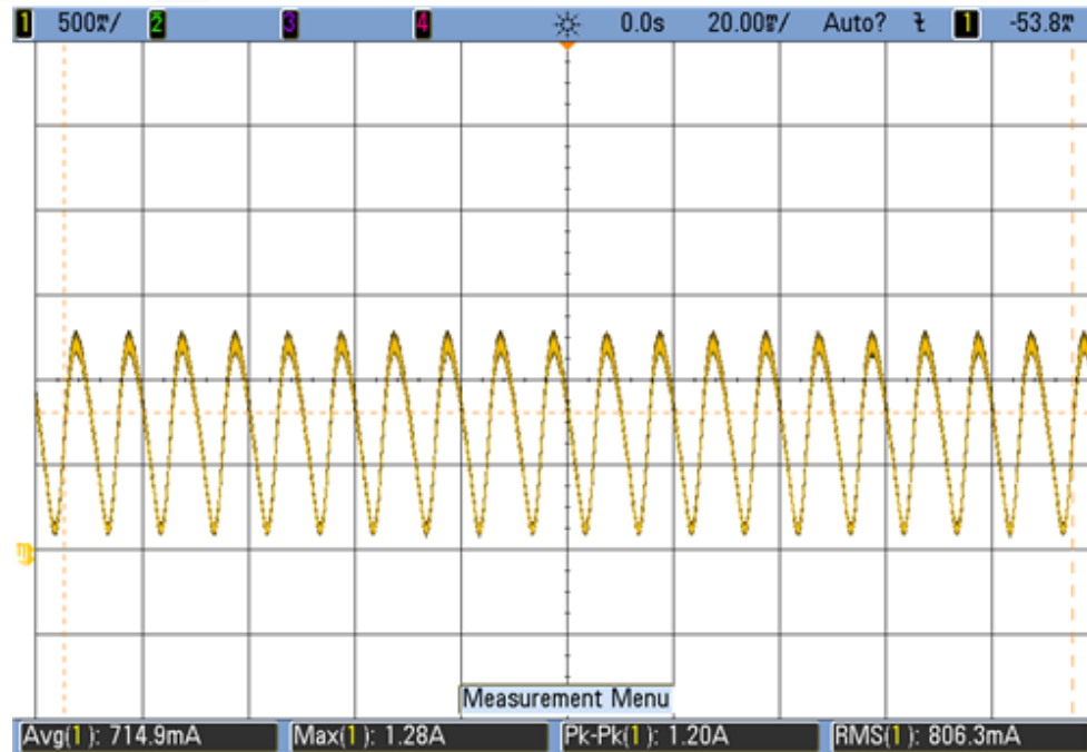
Figure 8: Ripple Current
