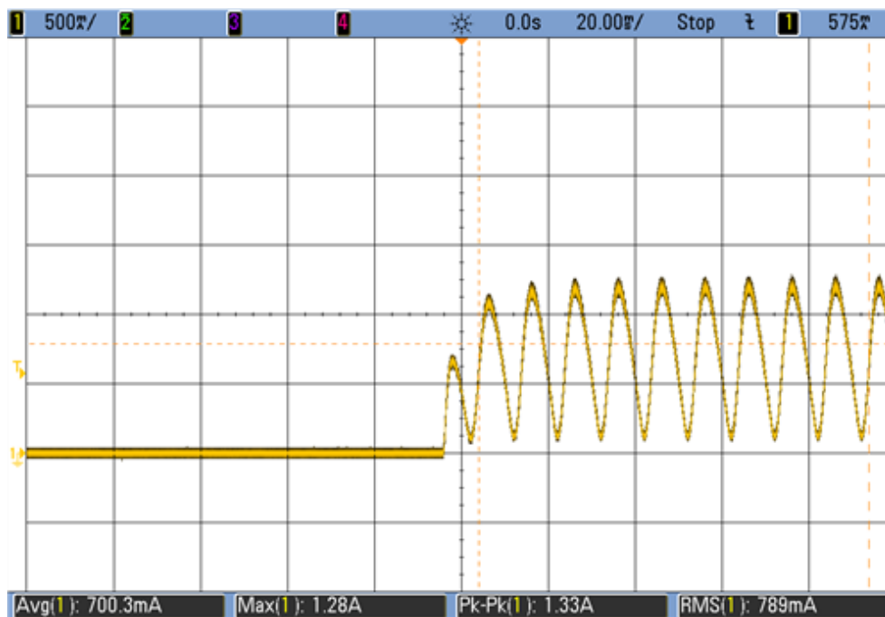
Figure 7: Initial turn-on (inrush) current
