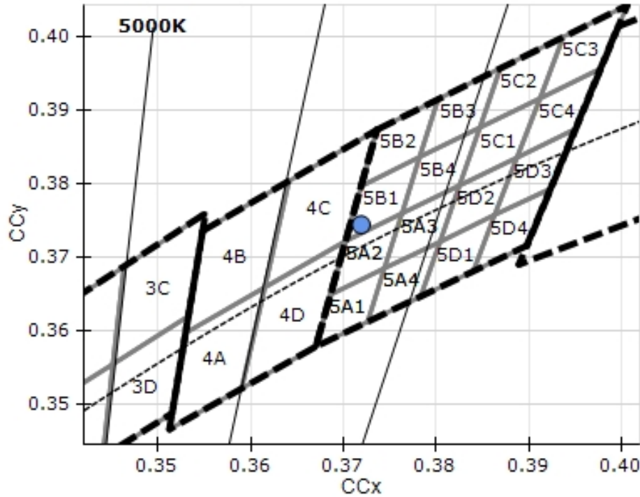
Chart 8: Measured Data Plotted on Cree Binning Chart
